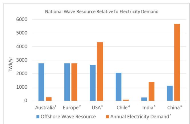
Fig. 2. Wave Energy Resource relative to Total Electricity Demand by Country. Offshore Wave Energy Resource data is presented, derived from (1) Hemer et al. [4]; (2) Clement et al. [57]; (3) EPRI [58]; (4) DCNS [59]; (5) Kumar and Anoop [60]; (6) Zhang et al. [61]. Electricity demand or production for each country is taken from the Global Energy Statistical Yearbook 2016 Enerdata [62].
