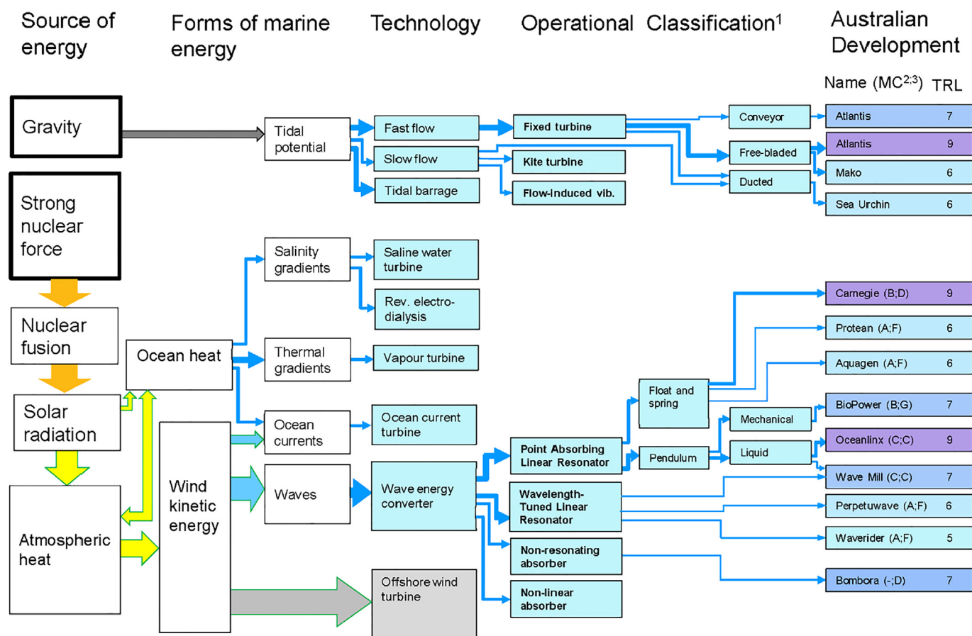
Fig. 3. Australian marine renewable energy developments, displaying Technological Readiness Levels (TRL's). 1 – Operational characterisation follows Manasseh et al. [25], 2 – The morphological classification codes follow Falcao [32]: A, oscillating body, floating; B, oscillating body, submerged; C, oscillating water column; and 3 – classification following Lopez et al. [33]: D, submerged pressure differential; E, overtopping; F, floating structure; G, oscillating wave surge converter.
